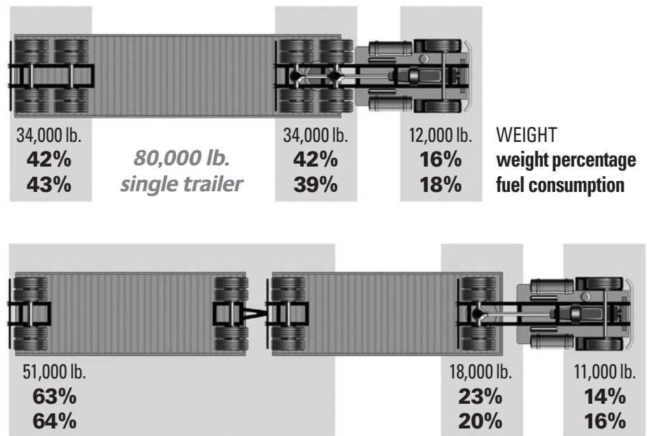
Axle Weight Distribution & Position Contribution to Fuel Economy
